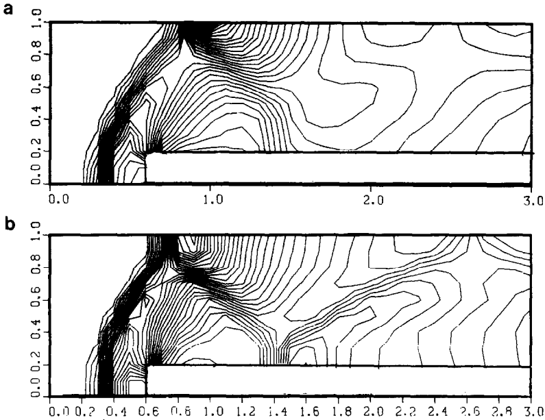
FIG. 9. Density contours with a 10 \times 30 grid for (a) the hybrid scheme (7.13) and (b) the ULTIC scheme.
