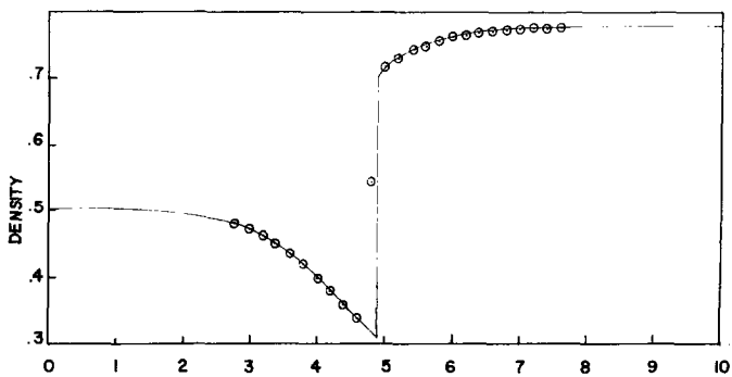
FIG. 7. ULT 1 scheme for (7.10) on a finer grid.
