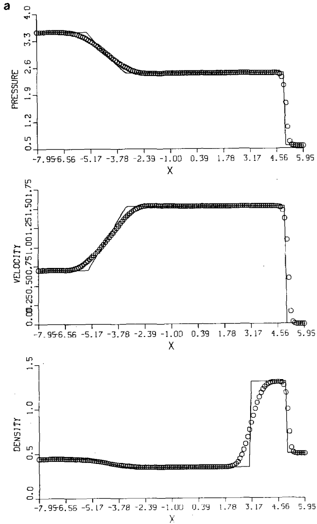
FIG. 2. (a) ROE scheme for (7.7); (b) LW scheme for (7.7); (c) ULT1 scheme for (7.7); (d) ULTIC scheme for (7.7).
