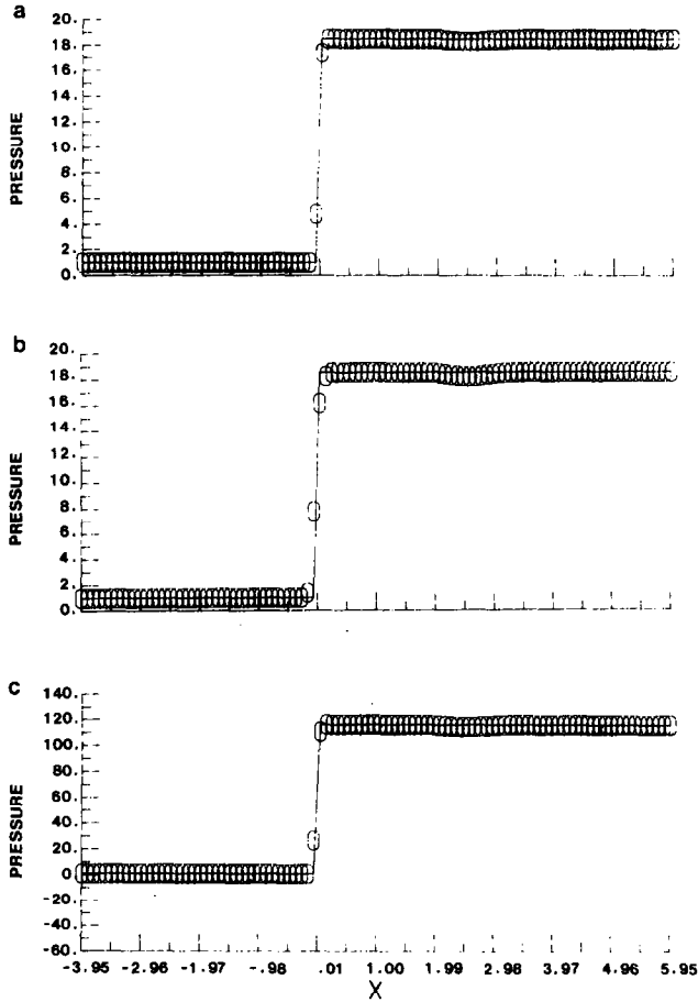
FIG. 4. ULT2 scheme with (a) \epsilon = 0.1 ( P_2/P_1 = 18.5 ), (b) \epsilon = 0.25 ( P_2/P_1 = 18.5 ), (c) \epsilon = 0.1 ( P_2/P_1 = 1.165 \times 10^2 ).
