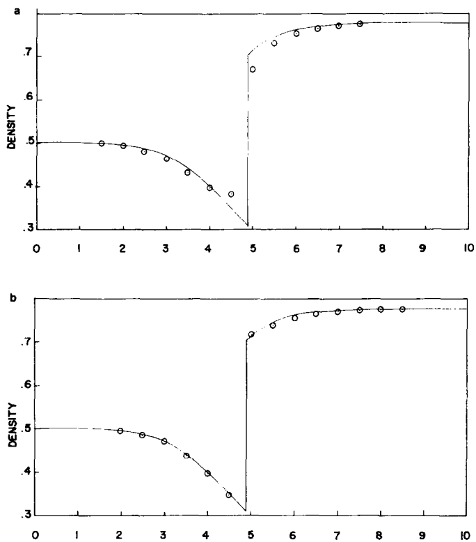
FIG. 6. (a) ROE scheme, (b) ULT 1 scheme for the divergent nozzle (7.10).
